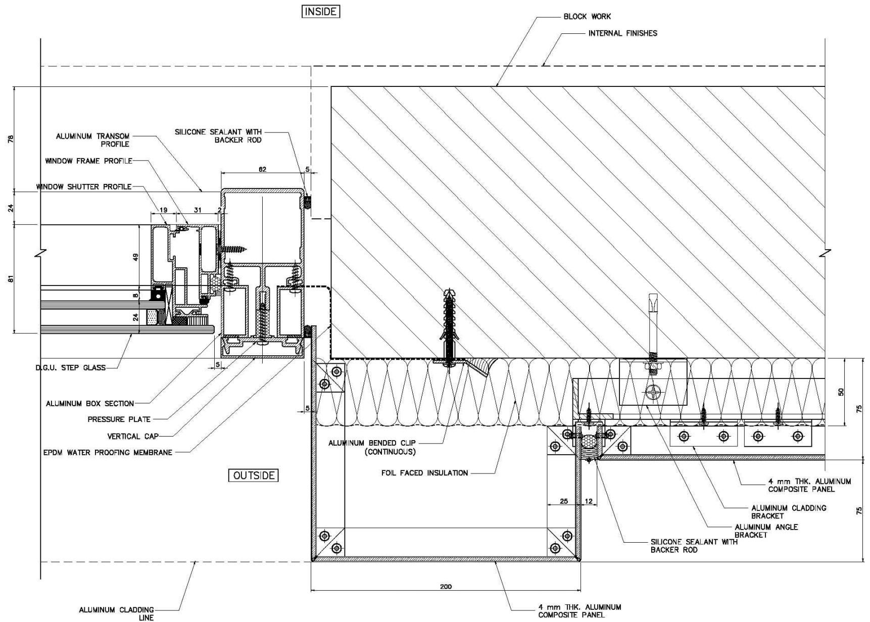
01 CORNER MULLION DETAIL SCALE 1:1
