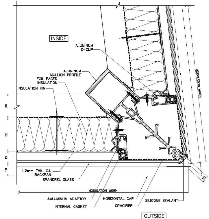
06 CORNER MULLION DETAIL SCALE 1:1
