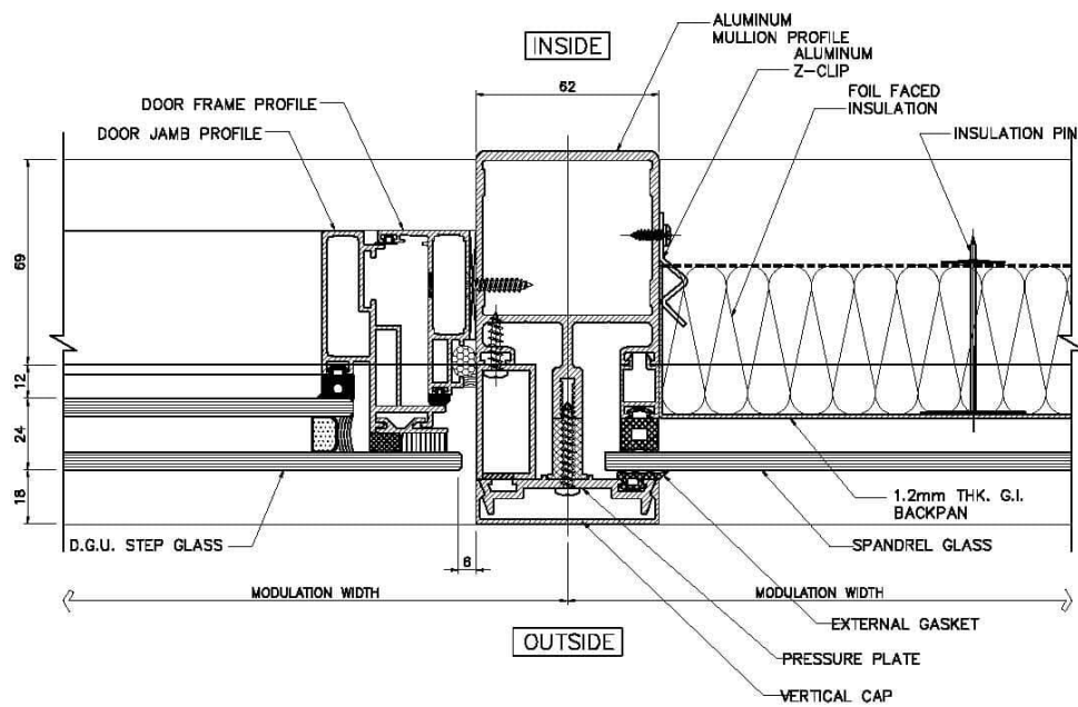
05 TYPICAL MULLION DETAIL SCALE 1:1
