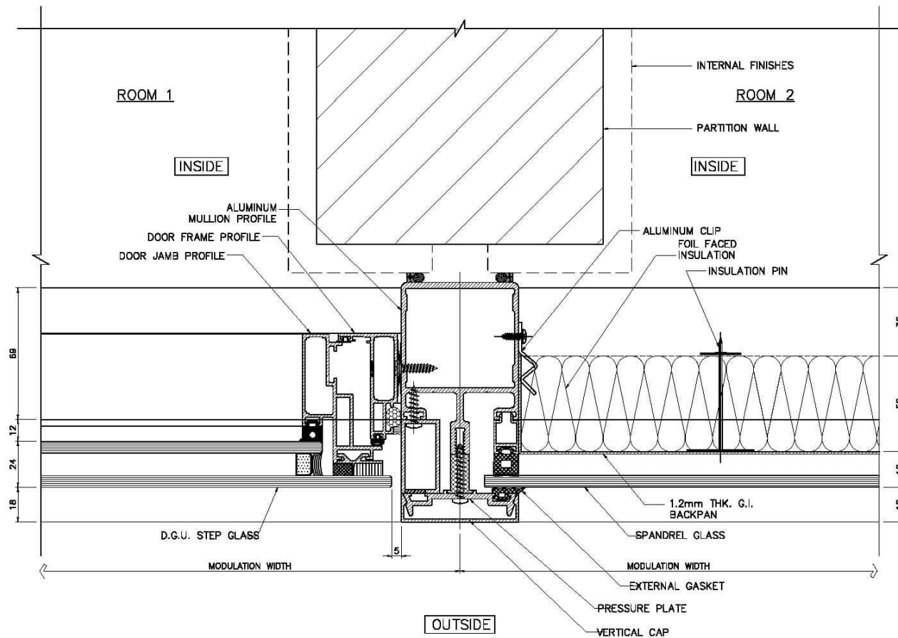
07 TYPICAL MULLION DETAIL SCALE 1:1
