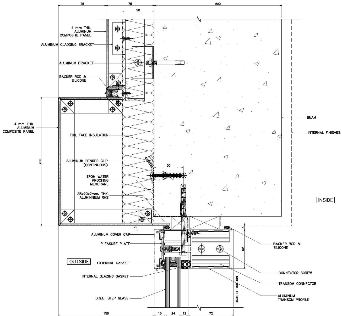
01 TOP TRANSOM DETAIL VISION AREA SCALE 1:1
