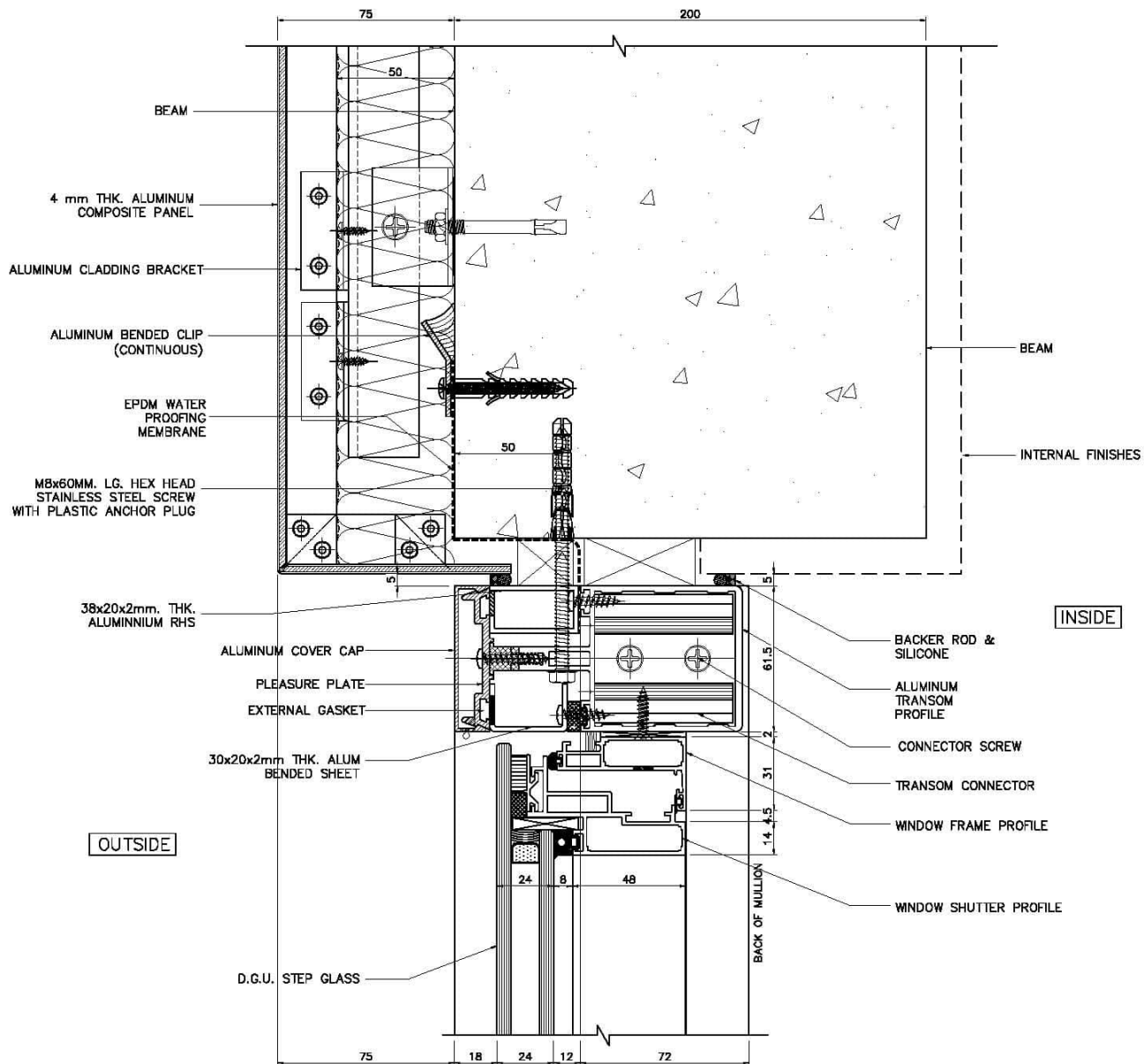
02 TOP TRANSOM WINDOW DETAIL SCALE 1:1
