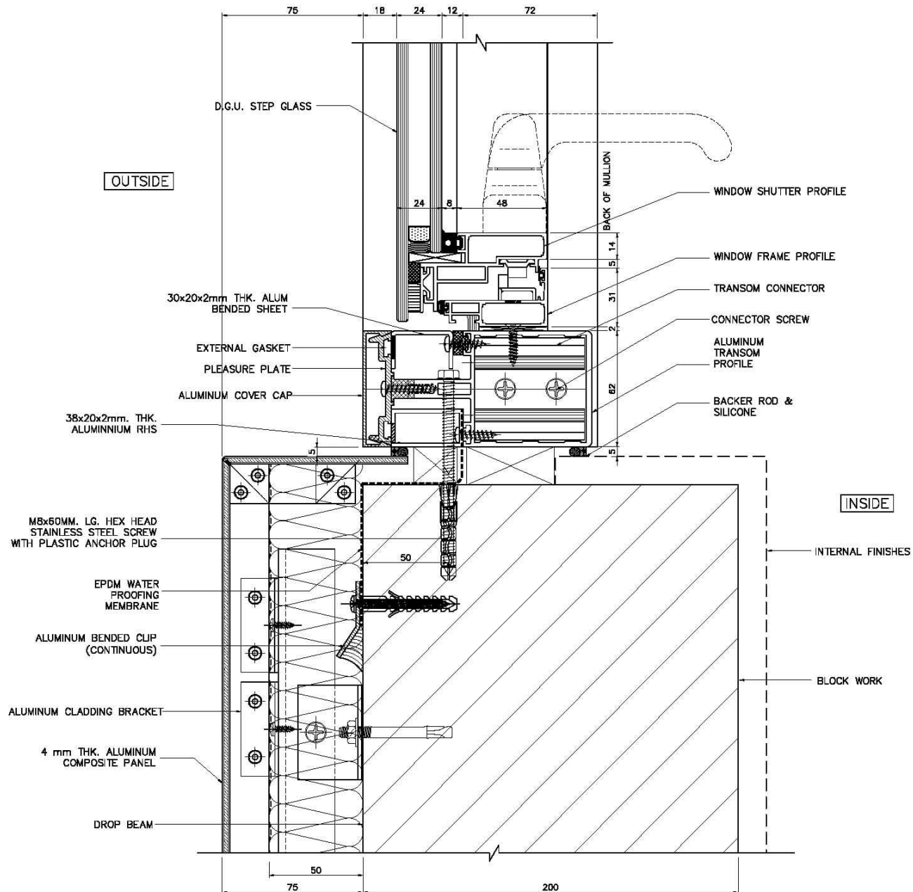
04 BOTTOM TRANSOM WINDOW DETAIL DT-002 SCALE 1:1
