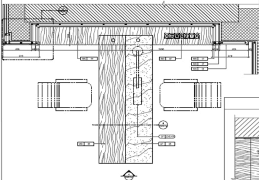
1 PLAN KITCHEN ISLAND SCALE: 1/4" = 1'-0"
