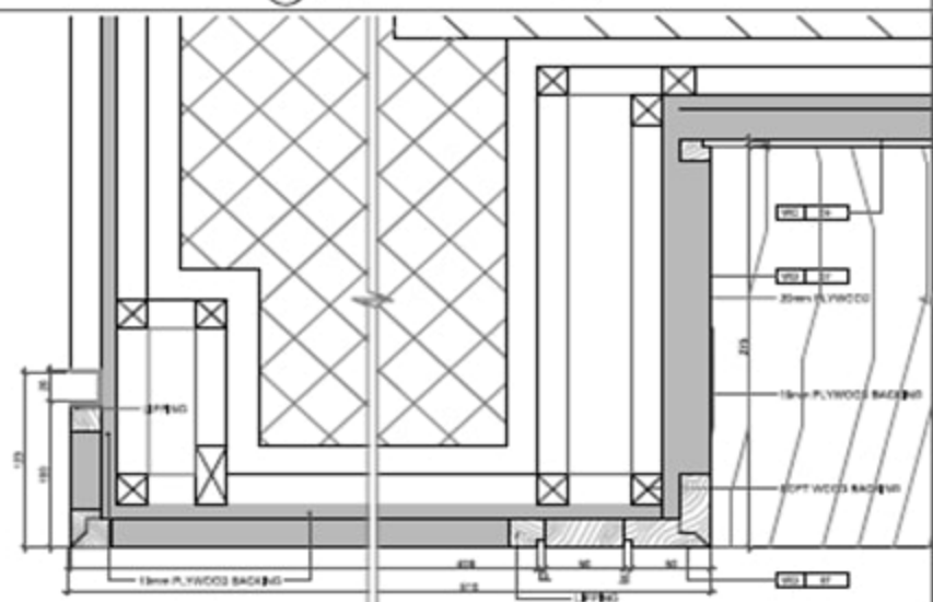
3 PLAN DETAIL KITCHEN ISLAND SCALE: 1/4" = 1'-0"
