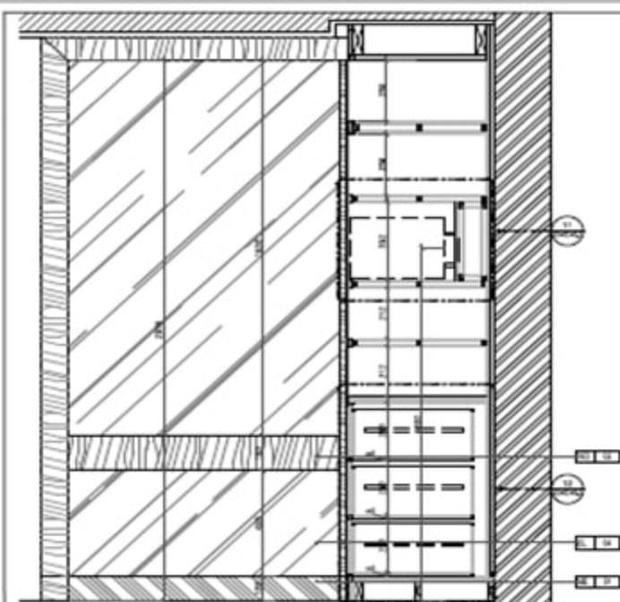
8 SECTION FACADE DETAIL SCALE 1/4"
