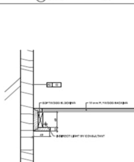
12 SECTION DETAIL FACADE DETAIL SCALE 1/4"
