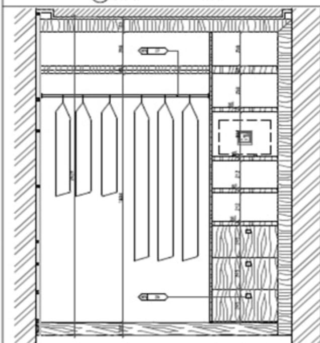
9 SECTION FACADE DETAIL SCALE 1/4"
