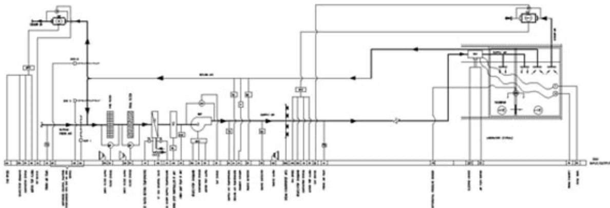
TYPICAL AMI CONTROL SYSTEM (TYPE-B)
