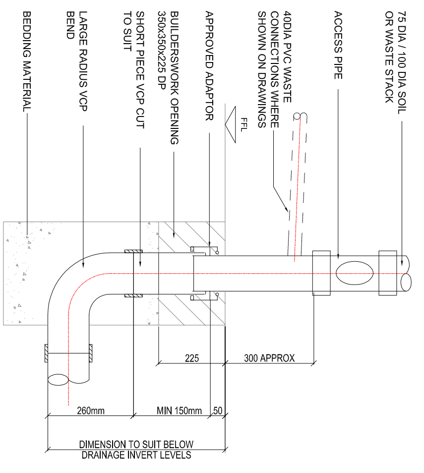
TYPICAL DETAIL FOR WASTE PIPES CONNECTING TO BELOW GROUND DRAINAGE DETAIL - A
