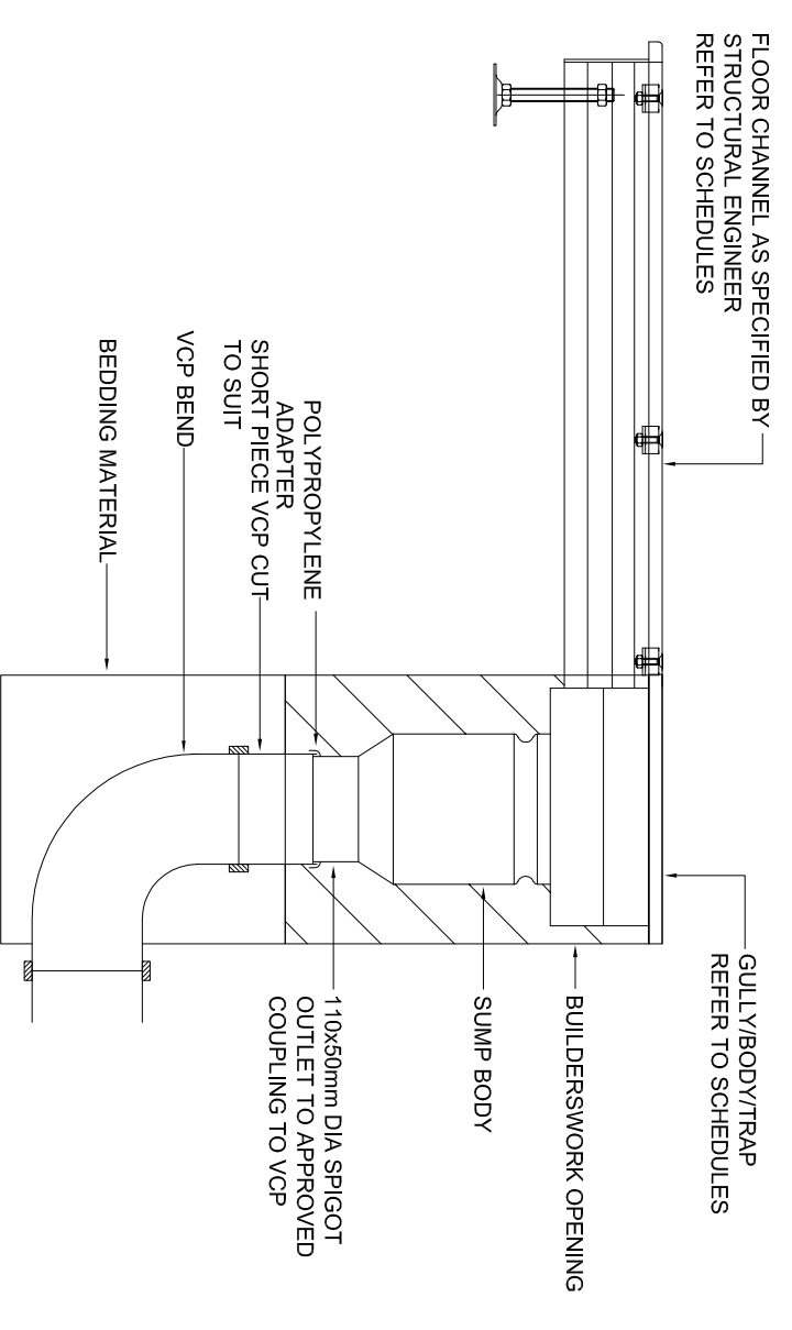
TYPICAL FLOOR CHANNEL/FLOOR GULLY DETAIL WITH INTEGRAL TRAPPED GULLY BODY DETAIL - E
