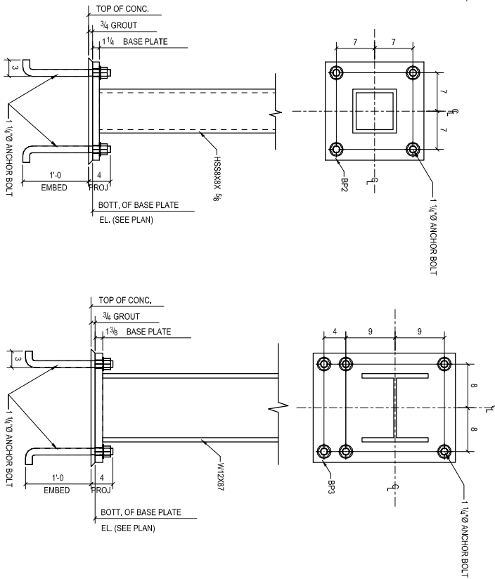
DETAIL 2 (REF: S-505) (12 LOCs) (ORIENTATION PER PLAN)
