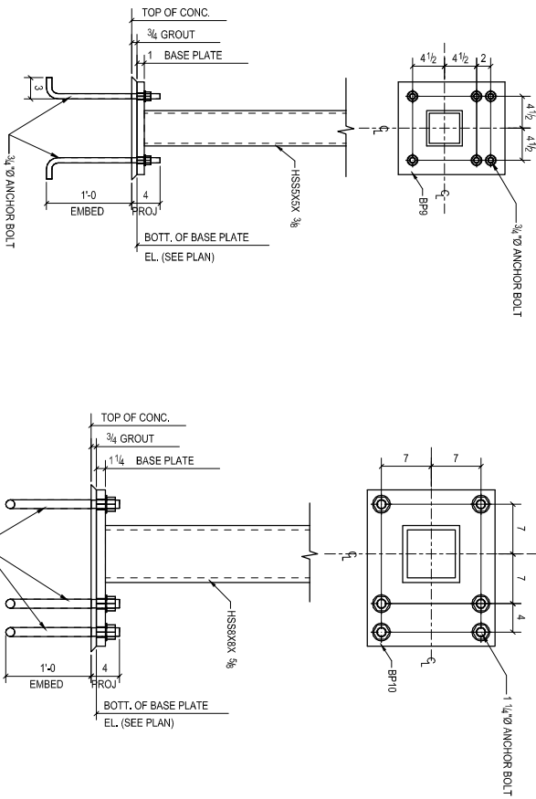
DETAIL 9 (REF: S-505) (22 LOCs) (ORIENTATION PER PLAN)
