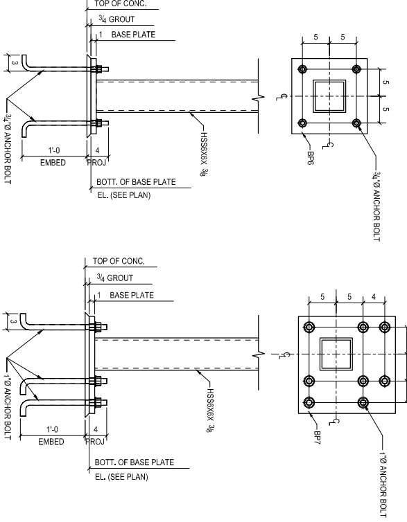
DETAIL 6 (REF: S-505) (07 LOCs) (ORIENTATION PER PLAN)
