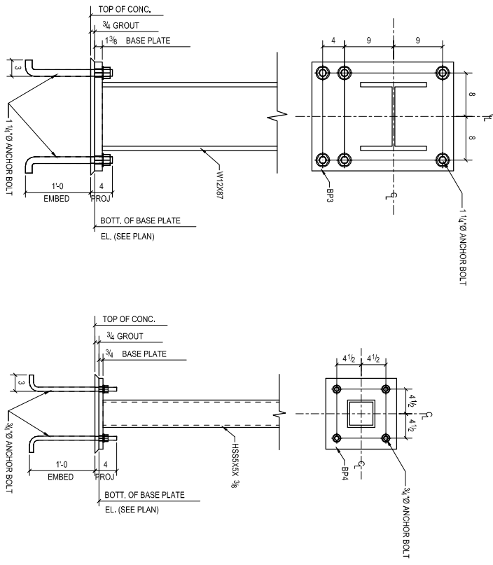
DETAIL 3 (REF: S-505) (01 LOCs) (ORIENTATION PER PLAN)
