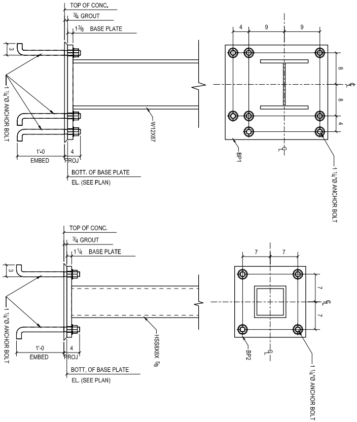
DETAIL 1 (REF: S-505) (01 LOCs) (ORIENTATION PER PLAN)
