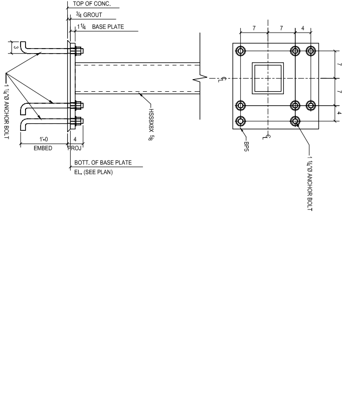
DETAIL 5 (REF: S-505) (17 LOCs) (ORIENTATION PER PLAN)
