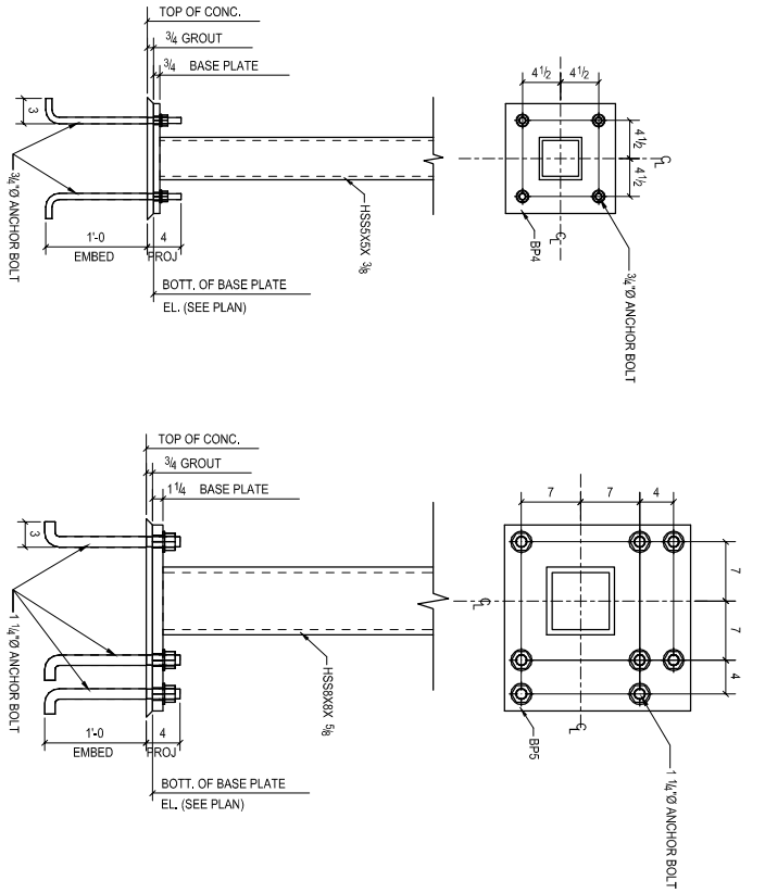
DETAIL 4 (REF: S-505) (115 LOCs) (ORIENTATION PER PLAN)
