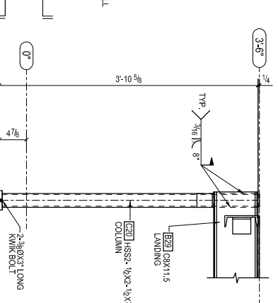
SECTION H SCALE 1:12
