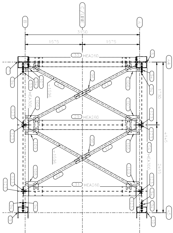
Plan +1620
