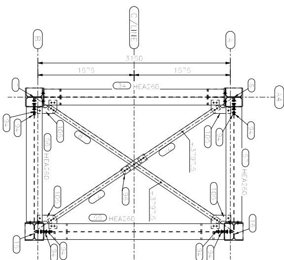
Plan +3820
