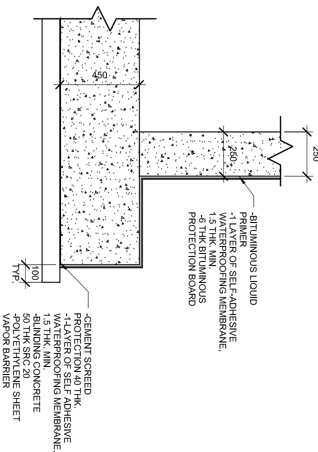
DETAIL-1
