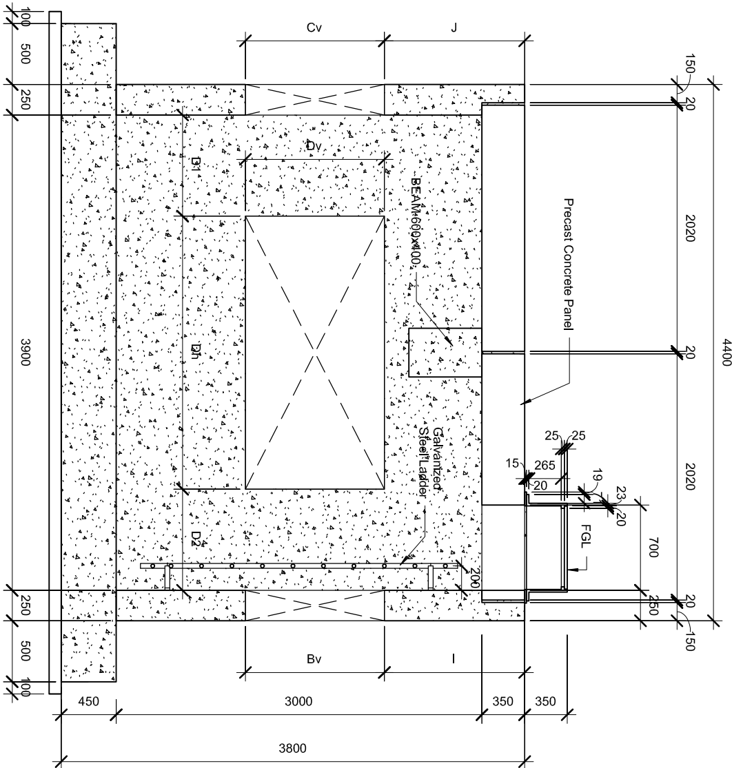
MH-T1-EL ELEVATION D
