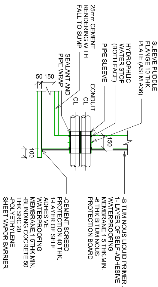
SECTION 4
