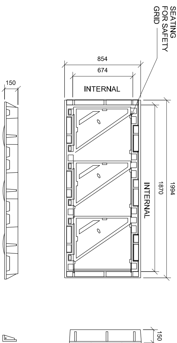
MANHOLE COVER
