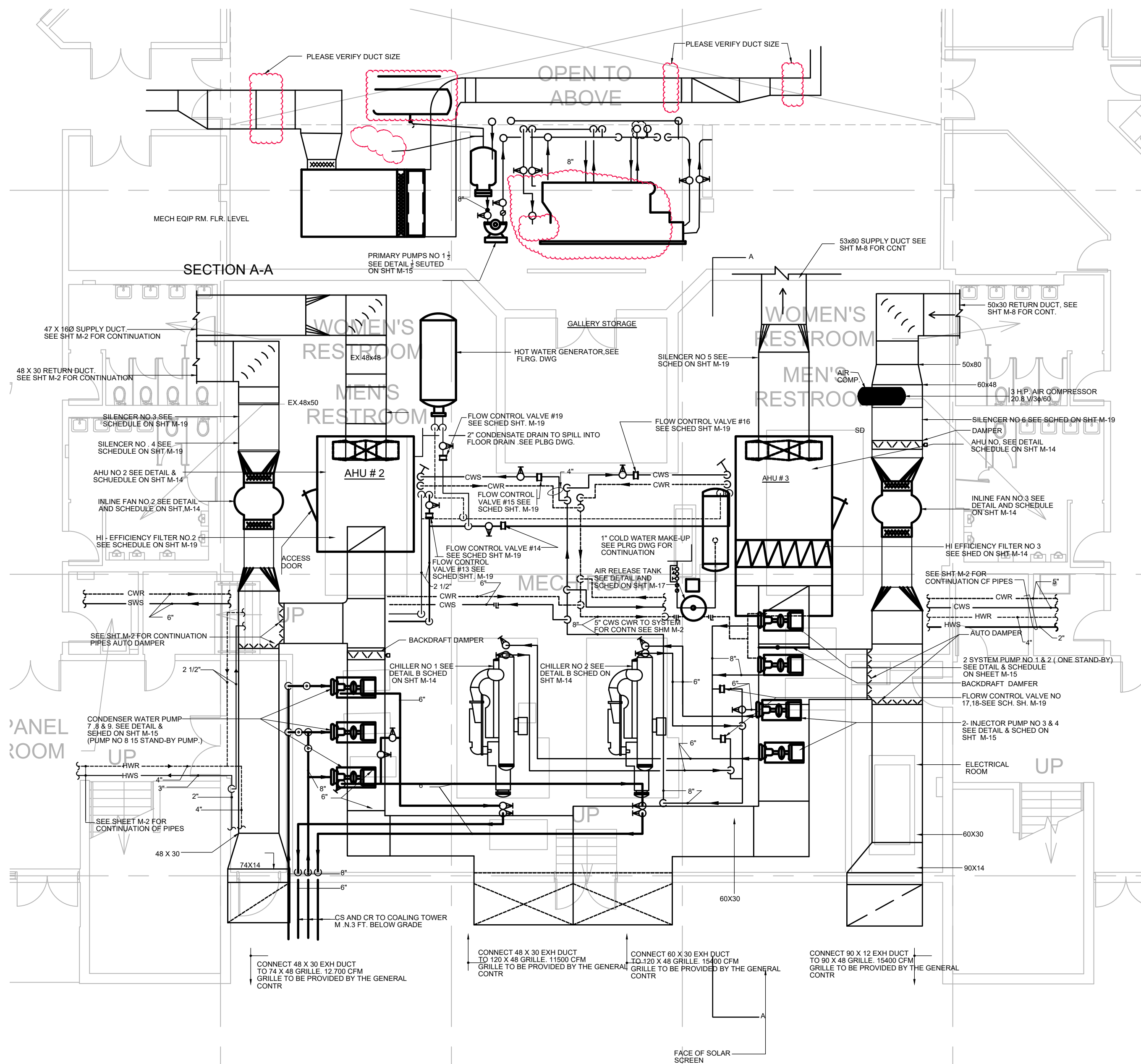
2 PART GROUND FLOOR PLAN - NEW WORK -MECHANICAL M-4 SCALE: 1/16"=1'-0"
