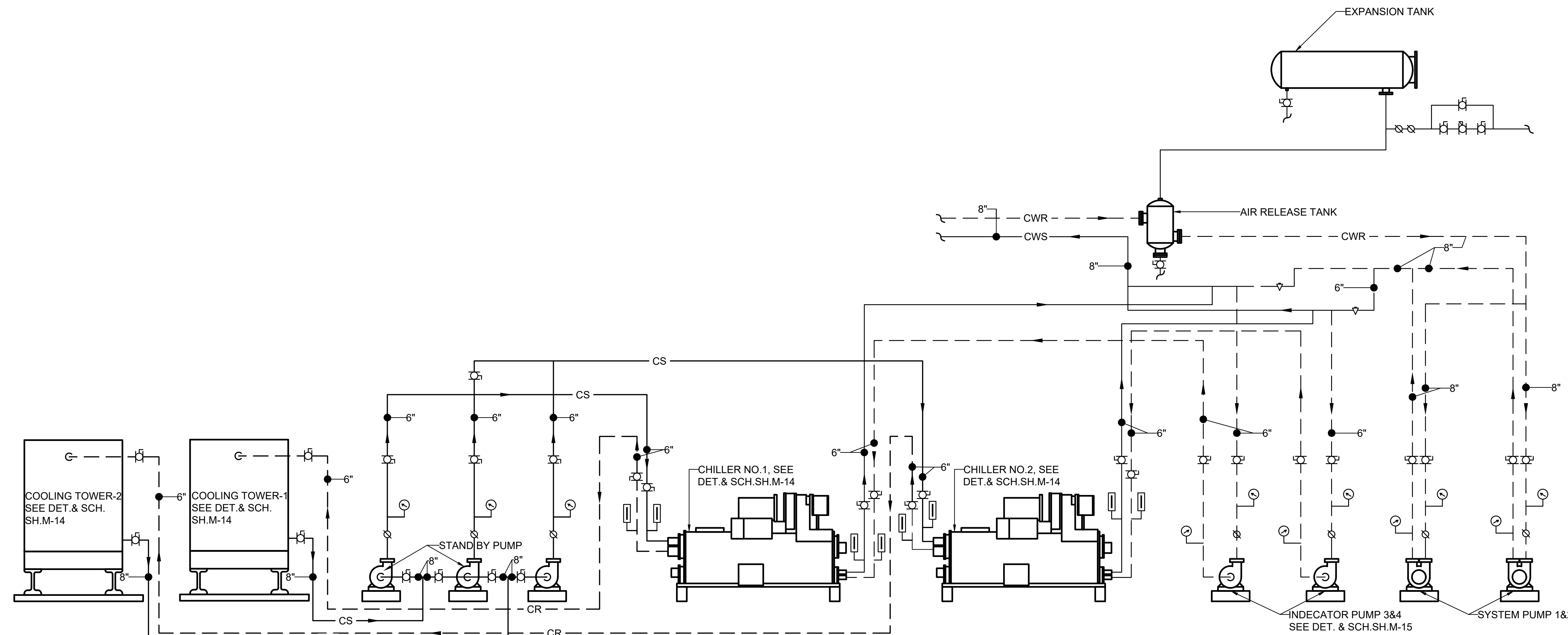
CHILLED WATER PIPING FLOW DIAGRAM
