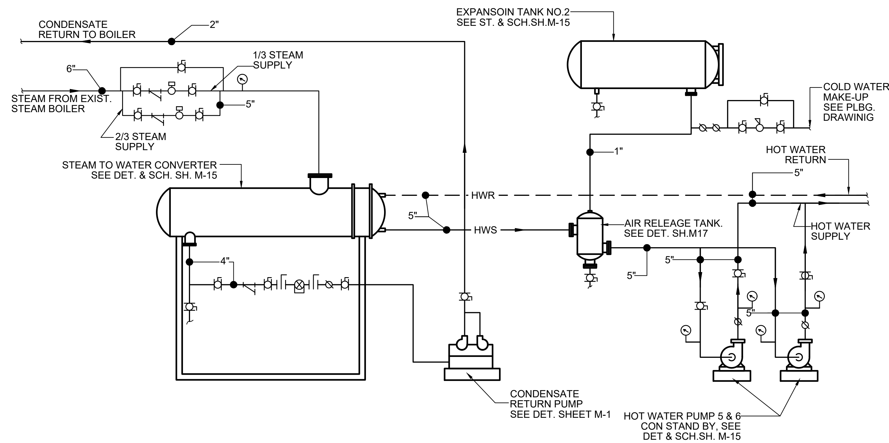
HOT WATER PIPING FLOW DIAGRAM
